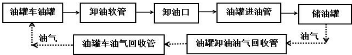
图2.4-3汽油卸油工艺流程框图
