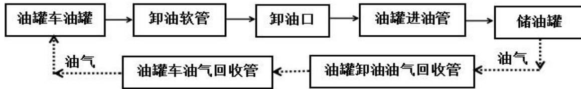
图2.4-3汽油卸油工艺流程框图
